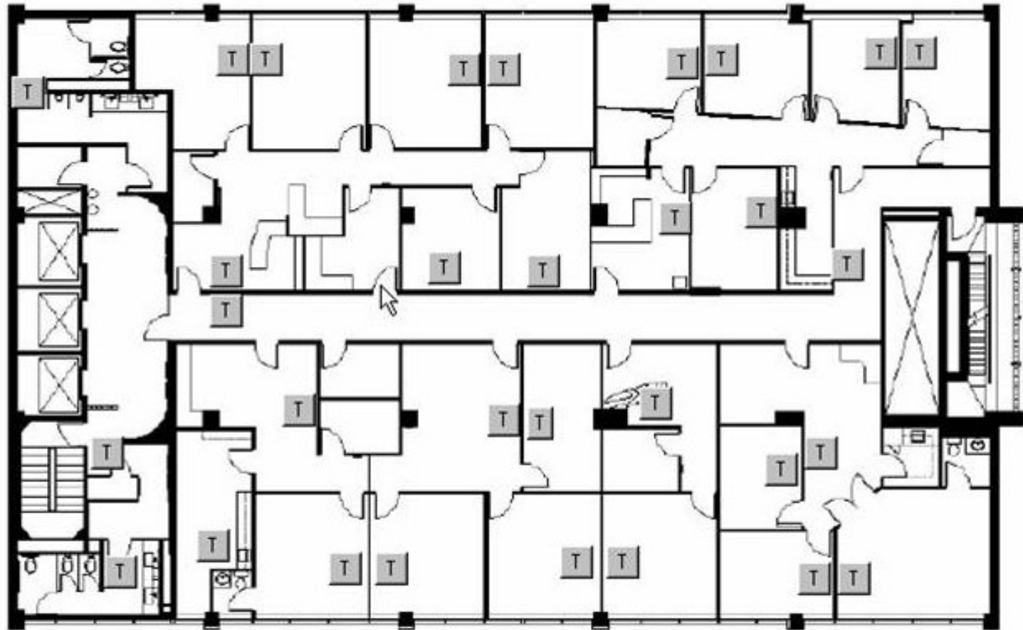
Thermostat Locations - 6th Floor
